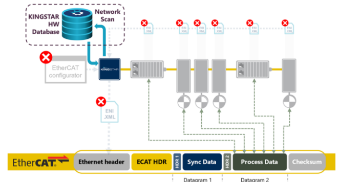
KINGSTAR Fieldbus Automatic configuration feature
